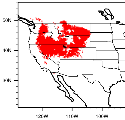
Diff (A2-Mod) artetrid
