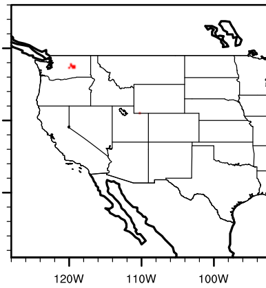
IPSL future artetrid
