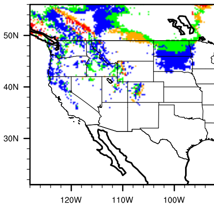
Diff (A2-Mod) amelalni
