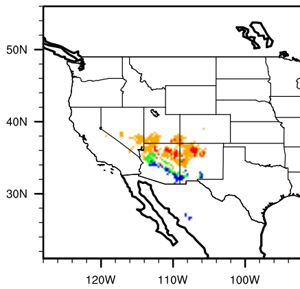
Diff (A2-Mod) alnuoblo
