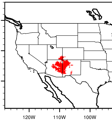
IPSL future alnuoblo
