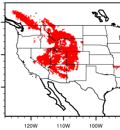
IPSL future acergran
