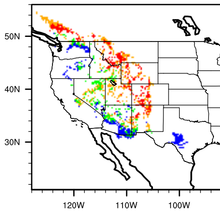
Diff (A2-Mod) acergran
